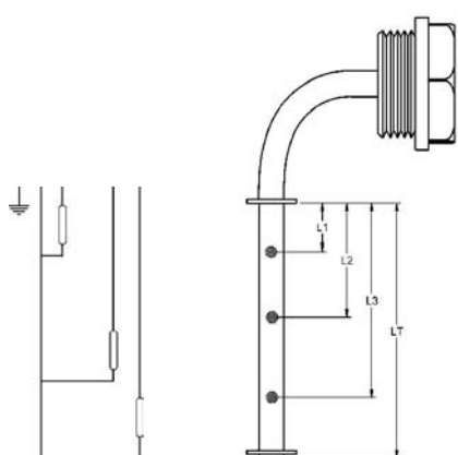
Basic electric connection
